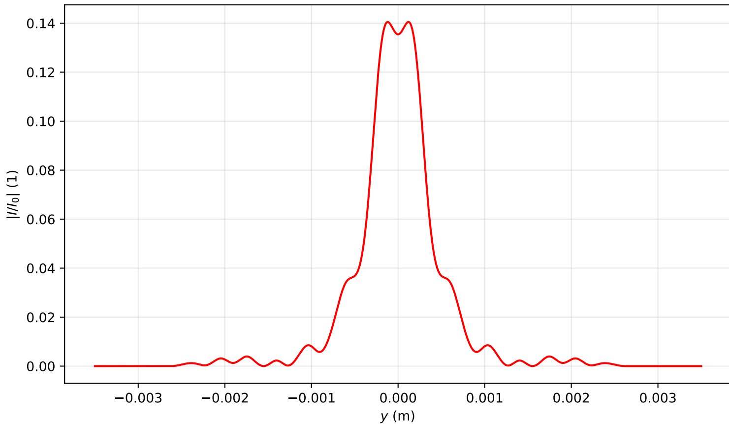
Intensity profile I(x=0, y, z=2.866)/I_0 , P_{in}=5.0P_{cr} , artificial time
